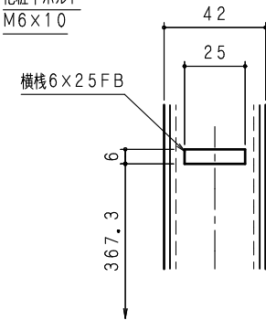
A部詳細 (S=1/2)
